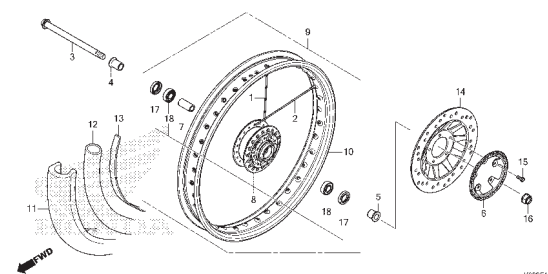
C-19.20 Roda Traseira
