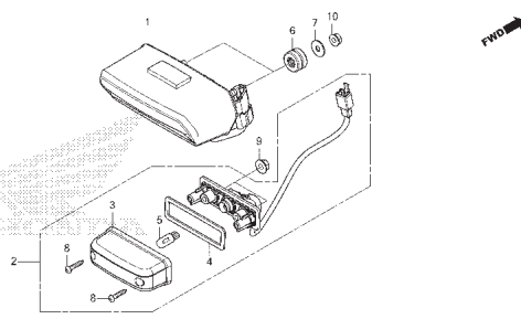
C-39 Chassi
