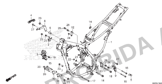
C-39 Chassi
